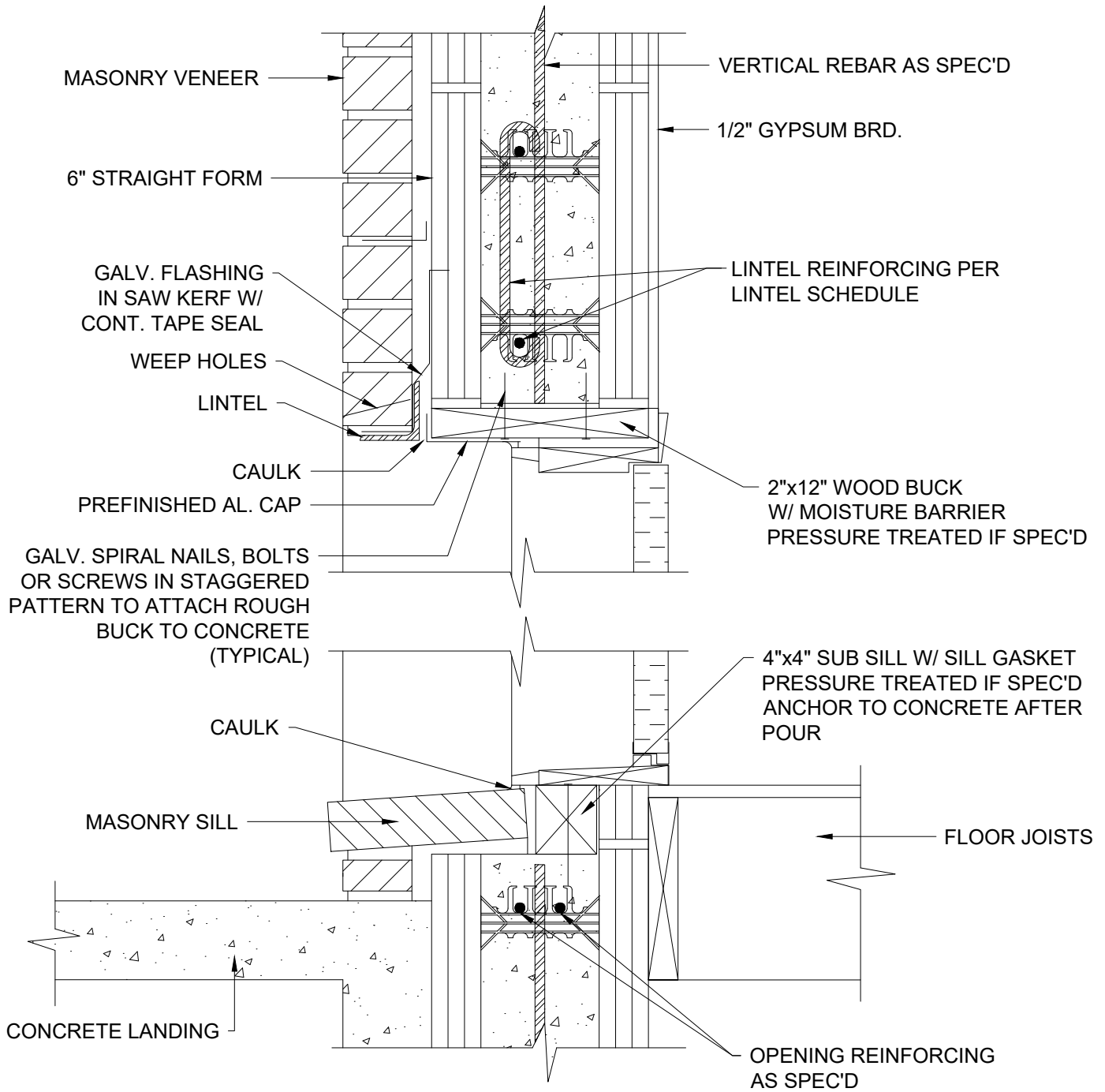
DOOR HEAD/SILL DETAIL 6 INCH
