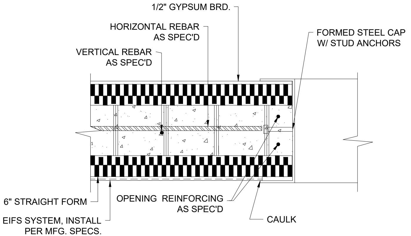
1 OVERHEAD DOOR JAMB DETAIL 6 INCH
