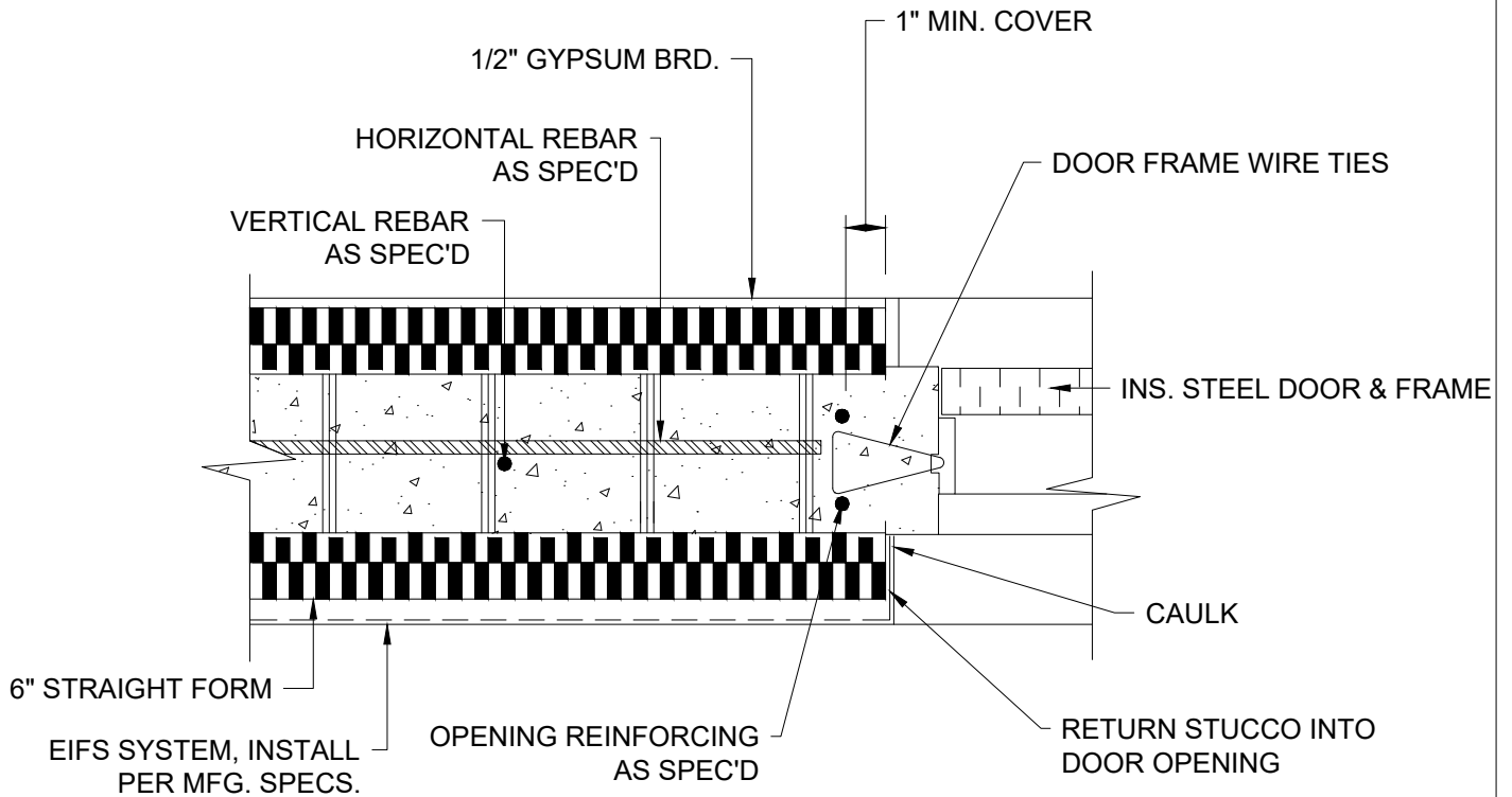
1 STEEL FRAME DOOR JAMB DETAIL 6 INCH
