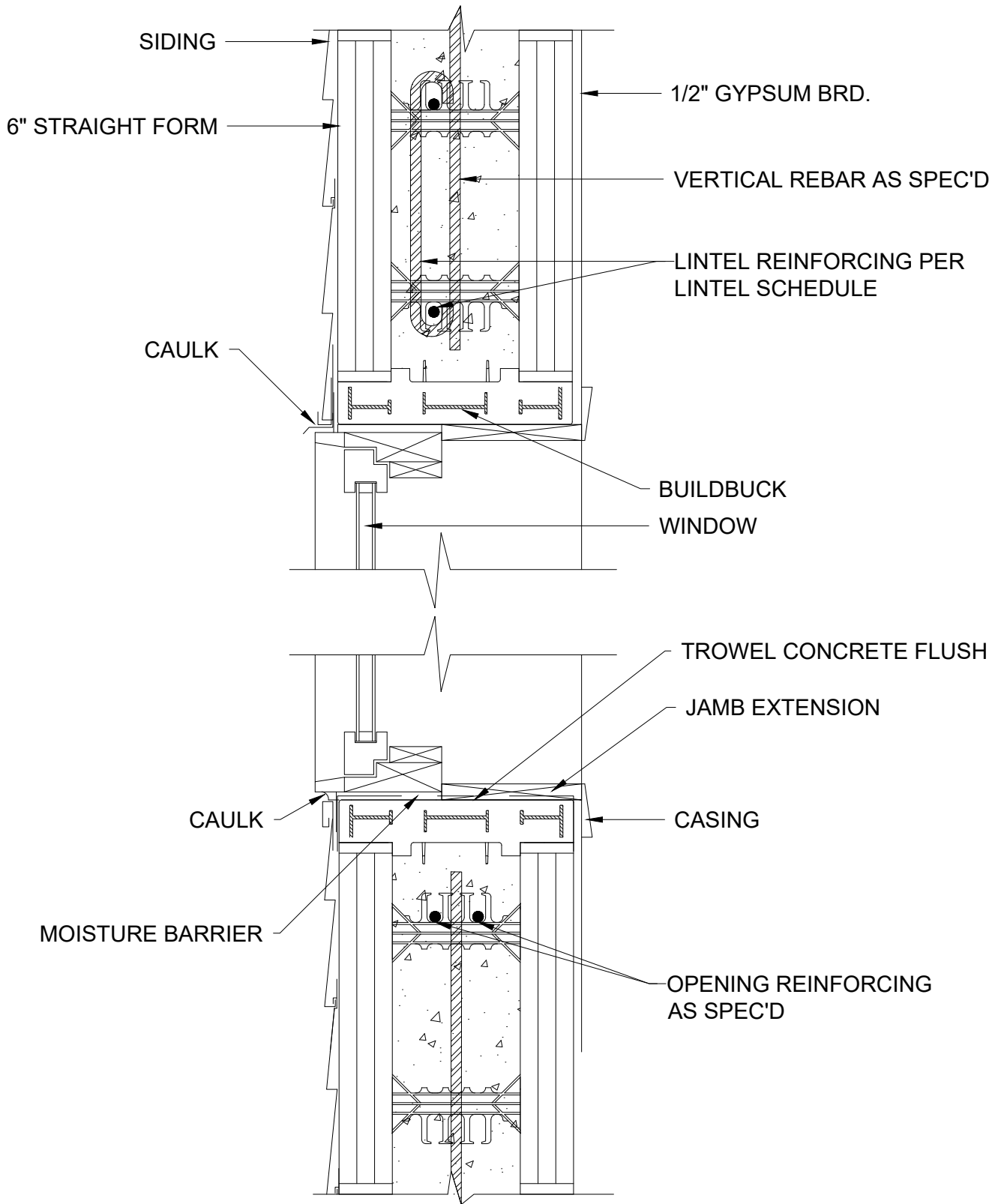
1 WINDOW HEAD/SILL DETAIL 6 INCH
