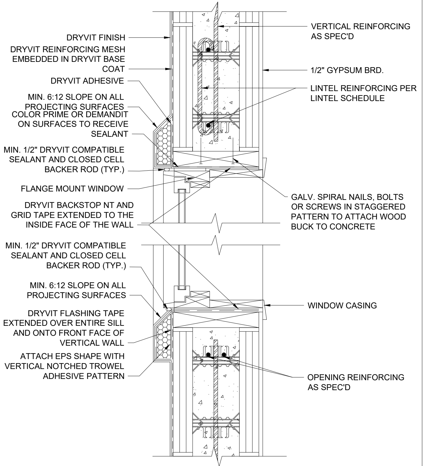
1 WINDOW HEAD/SILL DETAIL 6 INCH
