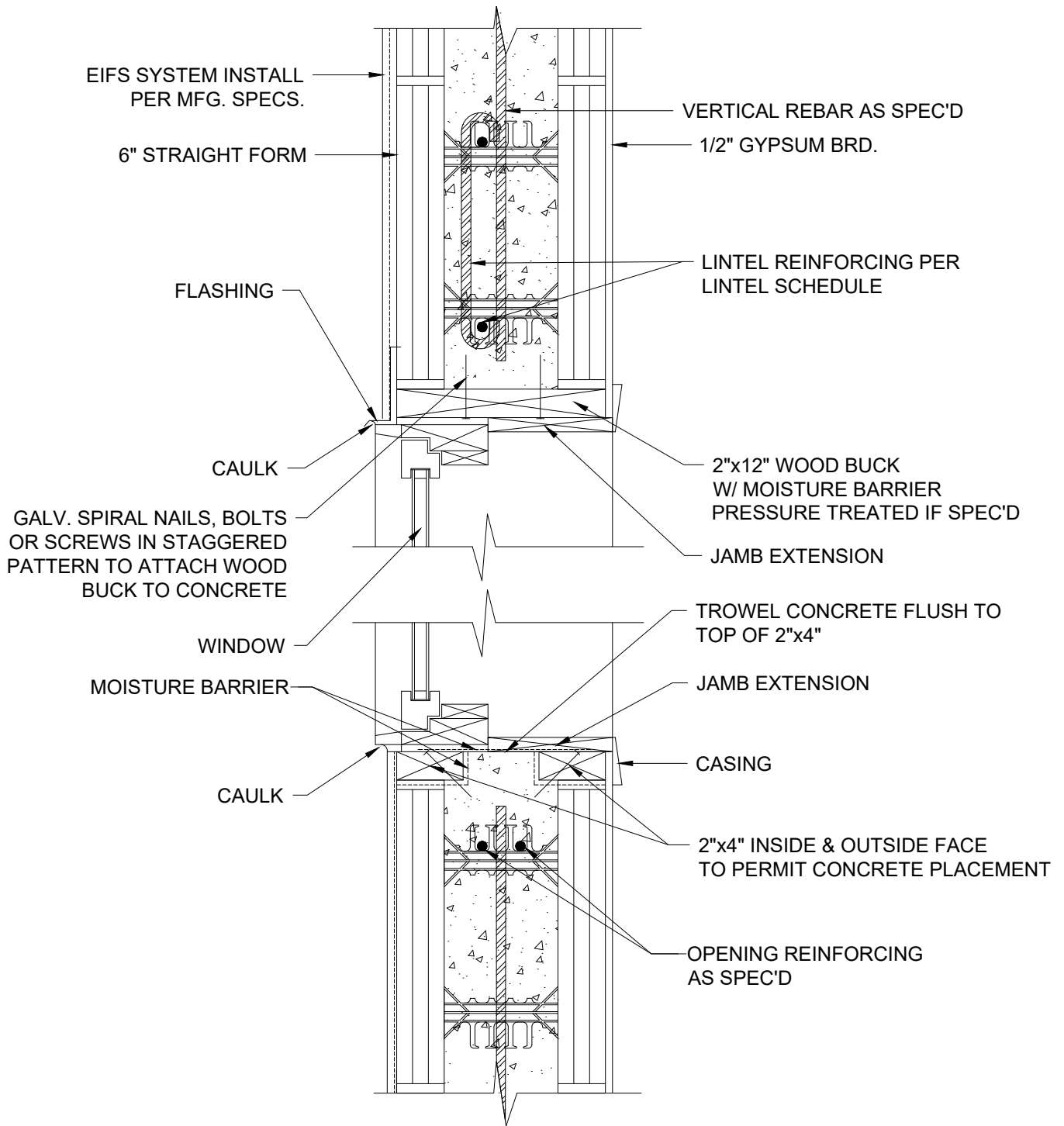
1 WINDOW HEAD/SILL DETAIL 6 INCH
