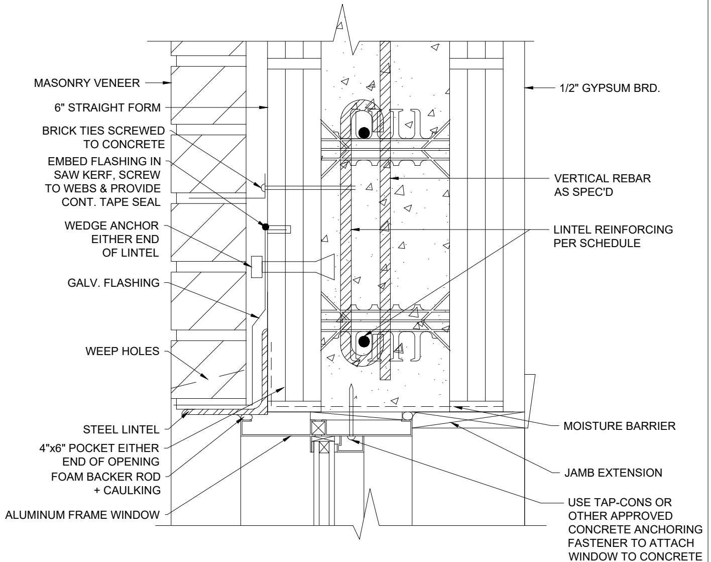
1 WINDOW HEAD DETAIL 6 INCH
