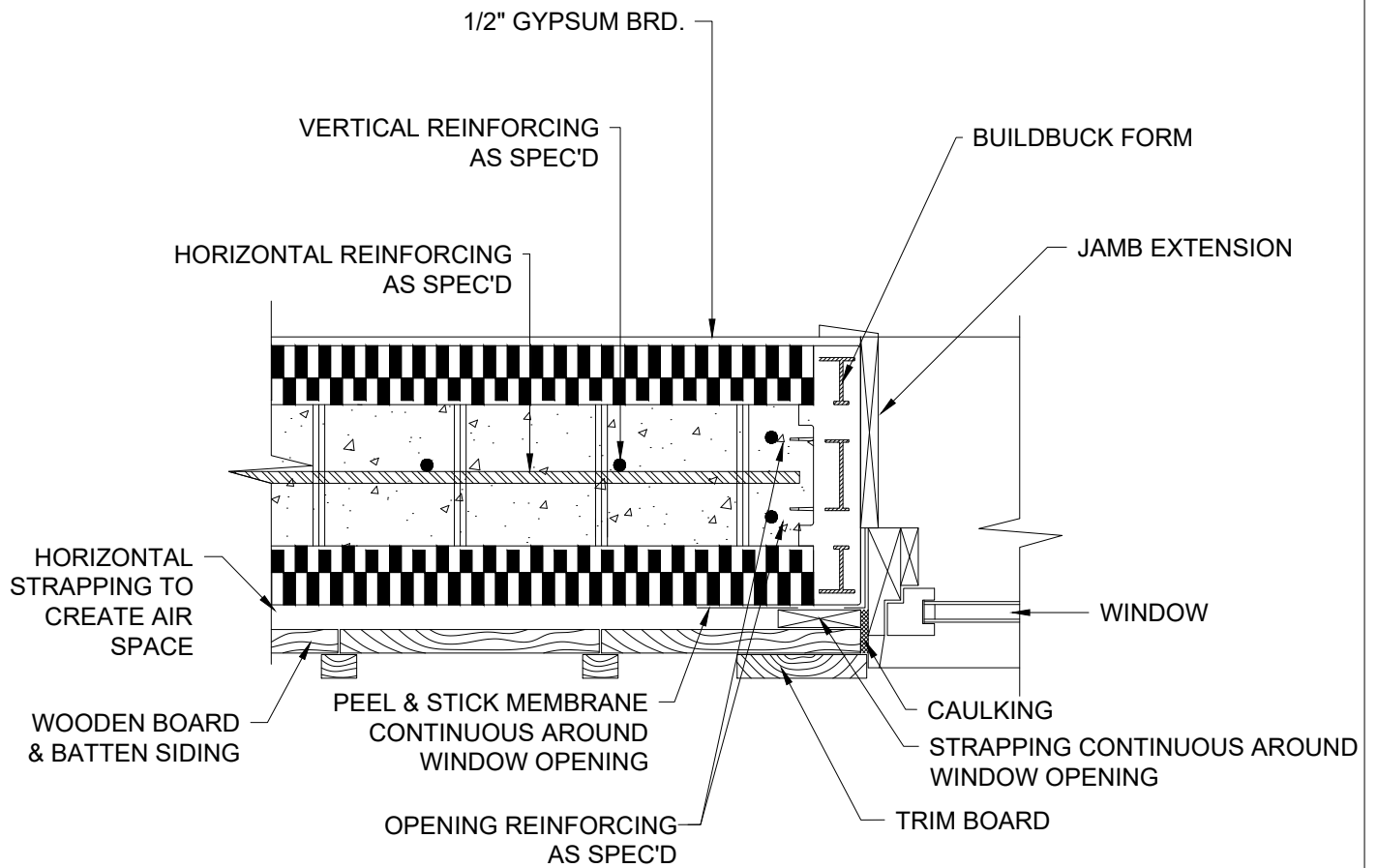
○ WINDOW JAMB DETAIL, BUILDBUCK, BOARD & BATTEN EXTERIOR 6 INCH
