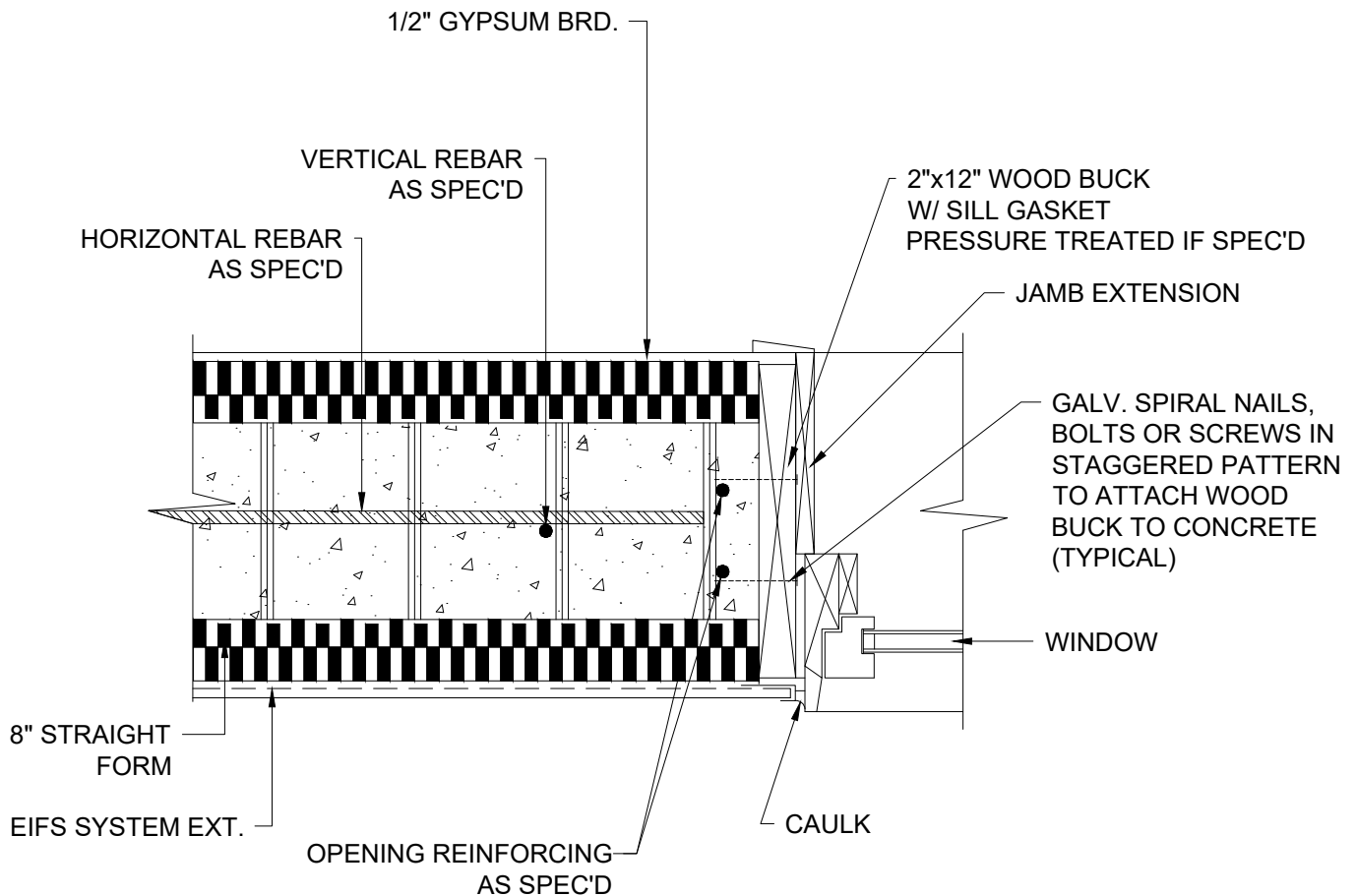
1 WINDOW JAMB DETAIL 8 INCH
