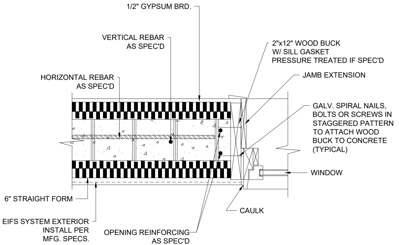
1 WINDOW JAMB DETAIL 6 INCH
