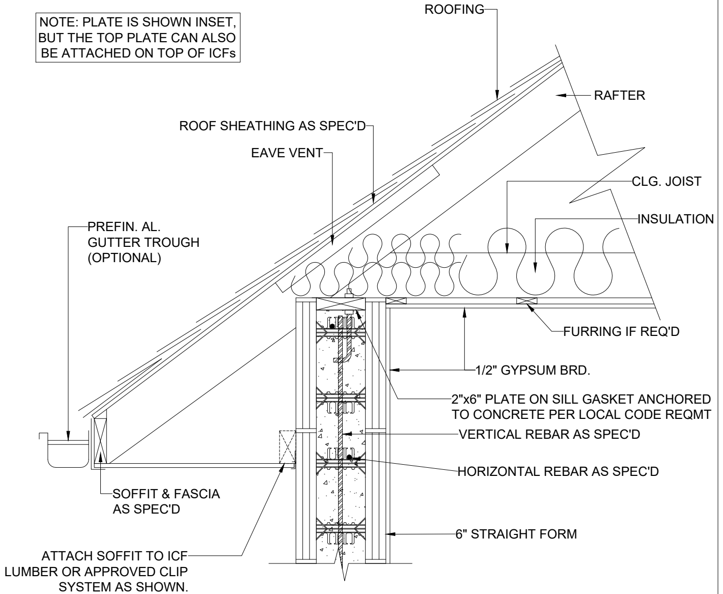
1 ROOF RAFTERS, LOW UPLIFT CONNECTION 6 INCH
