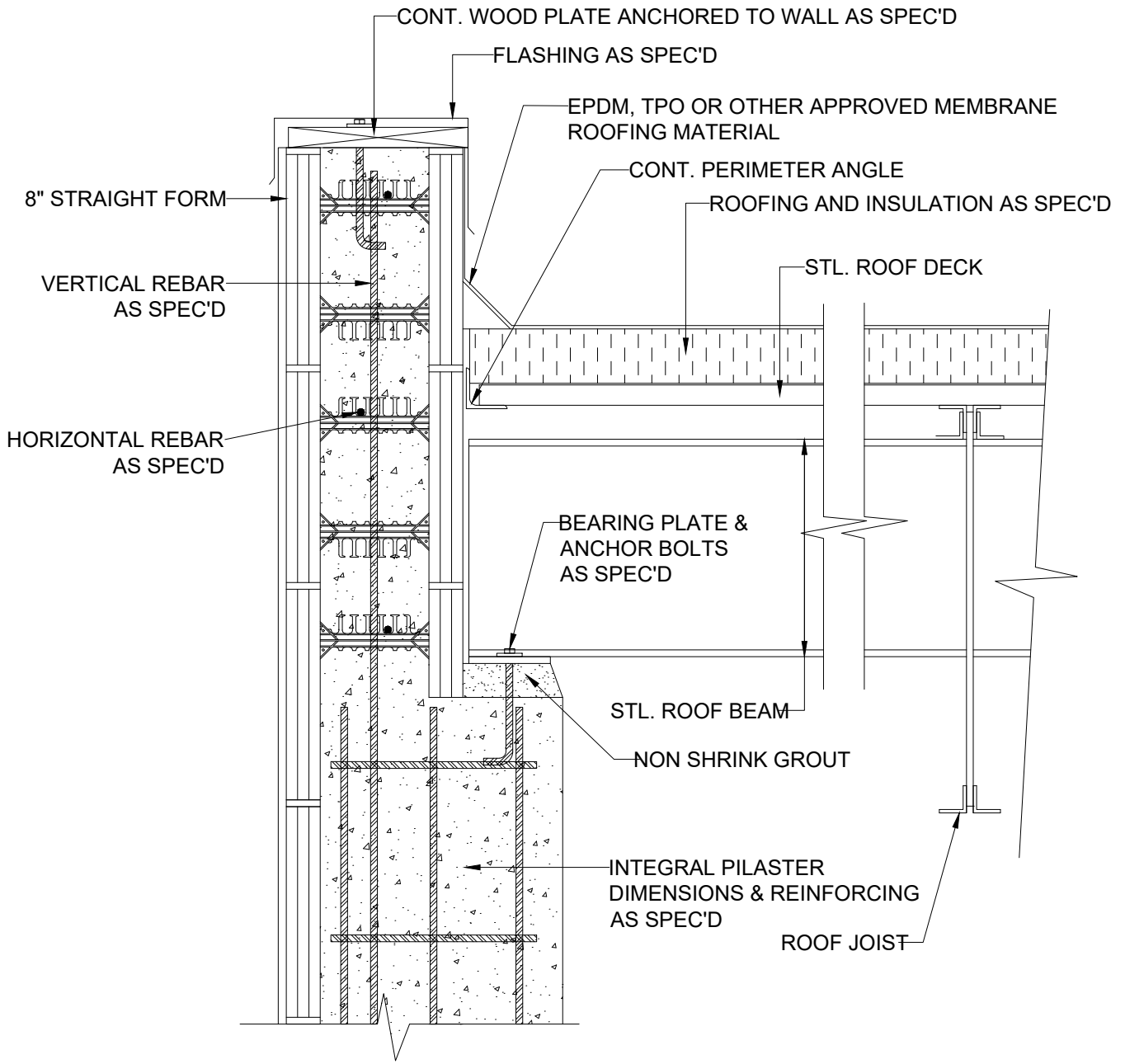
1 ROOM BEAM BEARING ON INTEGRAL PILASTER 8 INCH
