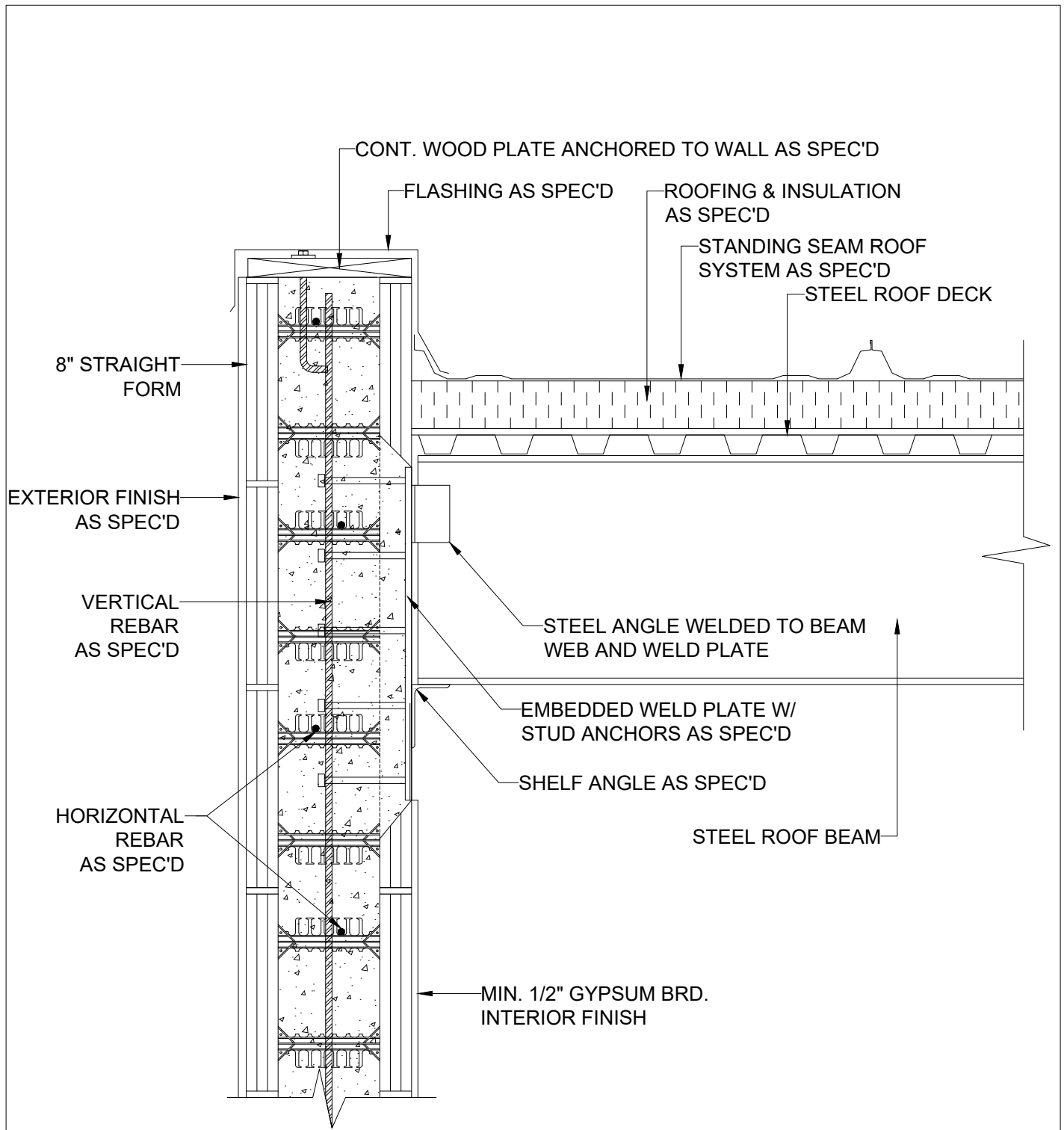
1 STEEL JOIST ROOF DETAIL BEARING WALL, BEAM FACE MOUNTED 8 INCH
