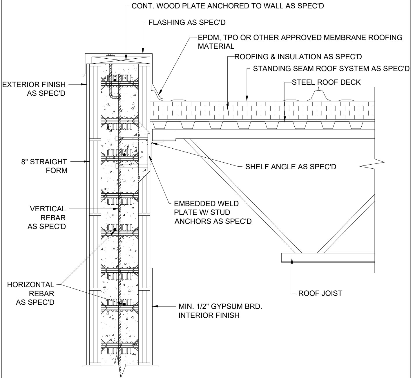
1 STEEL JOIST ROOF BEARING WALL JOISTS FACE MOUNTED 8 INCH
