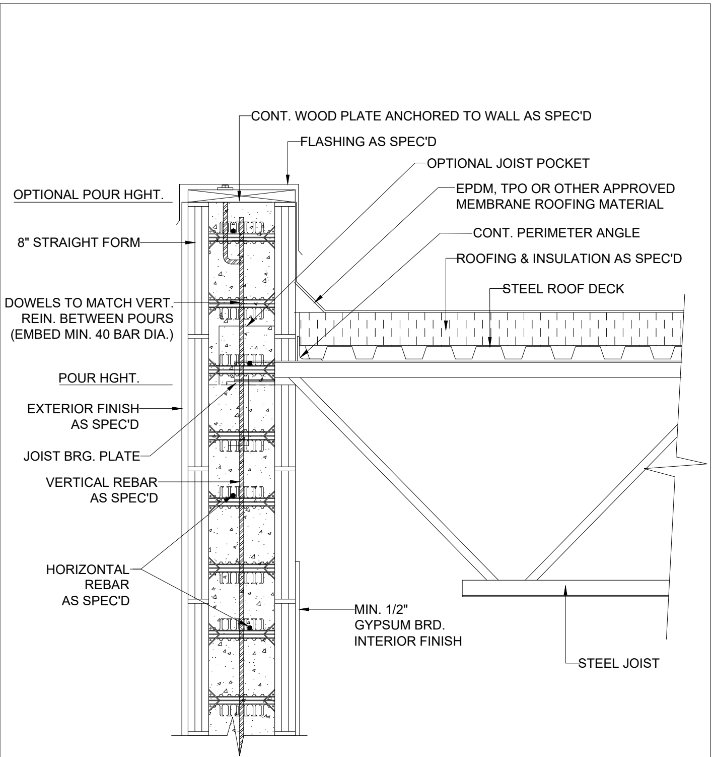
1 STEEL JOIST ROOF DETAIL BEARING WALL WITH PARAPET 8 INCH
