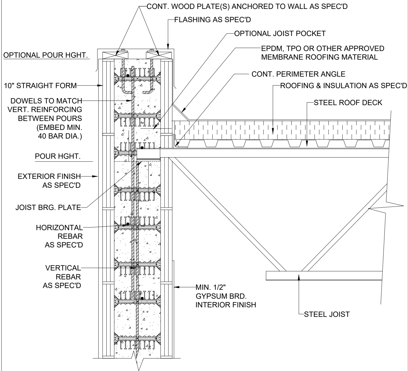
1 STEEL JOIST ROOF DETAIL BEARING WALL WITH PARAPET 10 INCH
