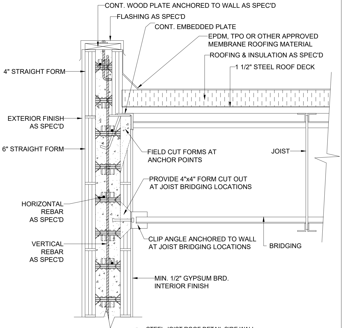
1 STEEL JOIST ROOF DETAIL SIDE WALL 6 INCH TO 4 INCH
