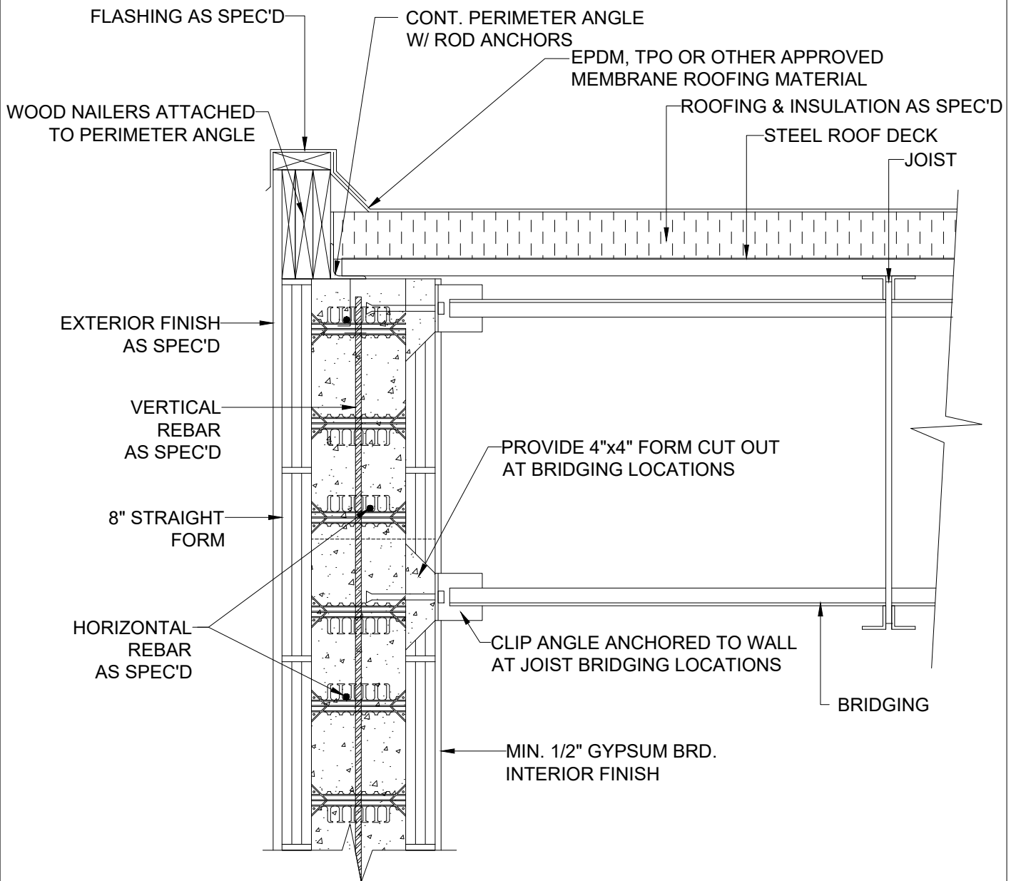
1 STEEL JOIST ROOF DETAIL SIDE WALL WITH NO PARAPET 8 INCH
