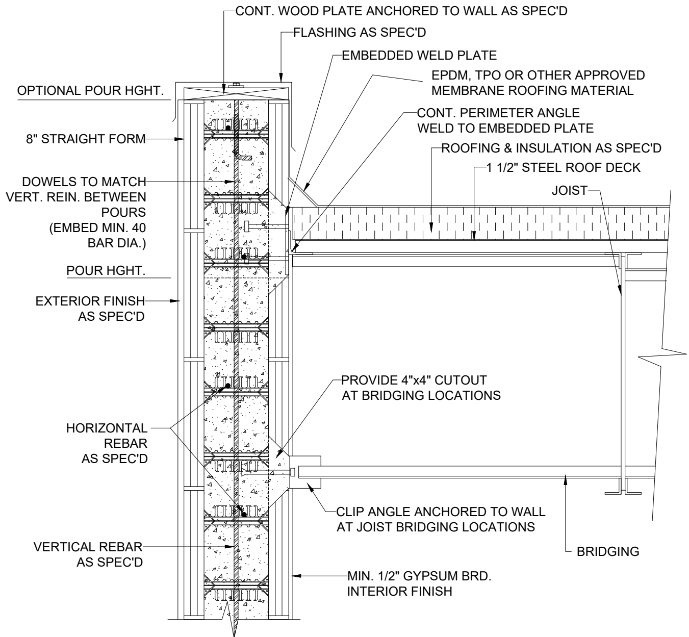
1 STEEL JOIST ROOF DETAIL SIDE WALL WITH PARAPET 8 INCH
