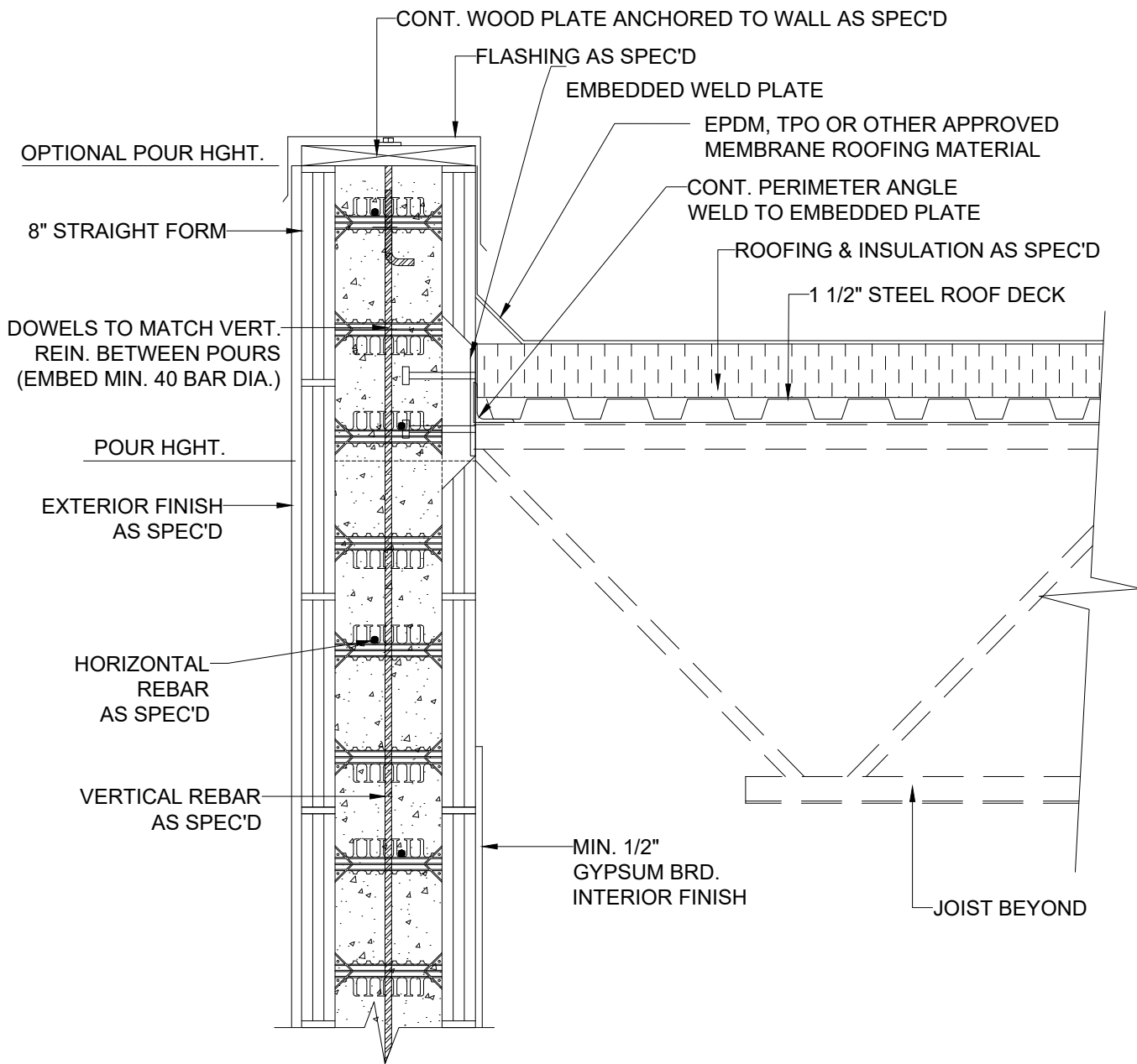
1 STEEL JOIST ROOF WITH PARAPET BETWEEN JOIST BEARING 8 INCH
