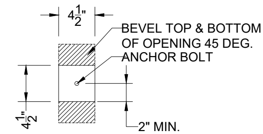
TYP. FORM CUTOUT
